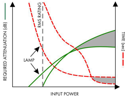
Typical Loudspeaker Power Handling Performance Overlaid with a lamp
