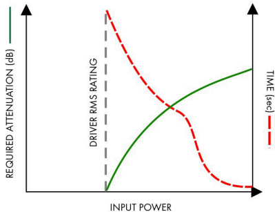
Typical Loudspeaker Power Handling Performance
