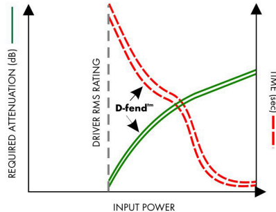
Typical Loudspeaker Power Handling Performance Overlaid with D-fend™
